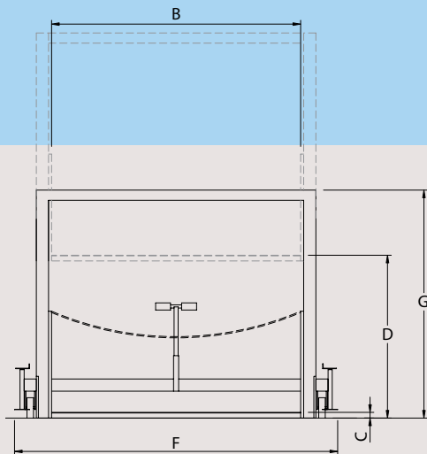
General Dimensions (mm) (Alternative machine dimensions also available)
